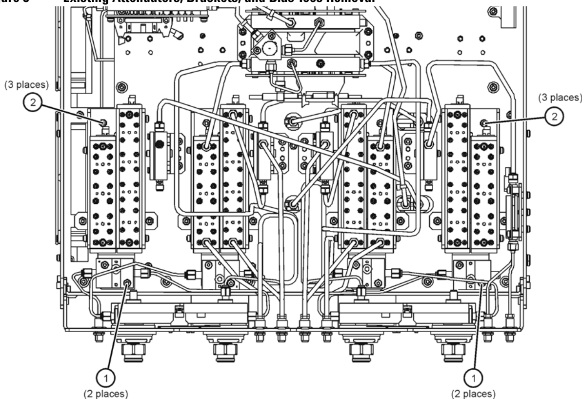
Figure 5 Existing Attenuators, Brackets, and Bias Tees Removal
