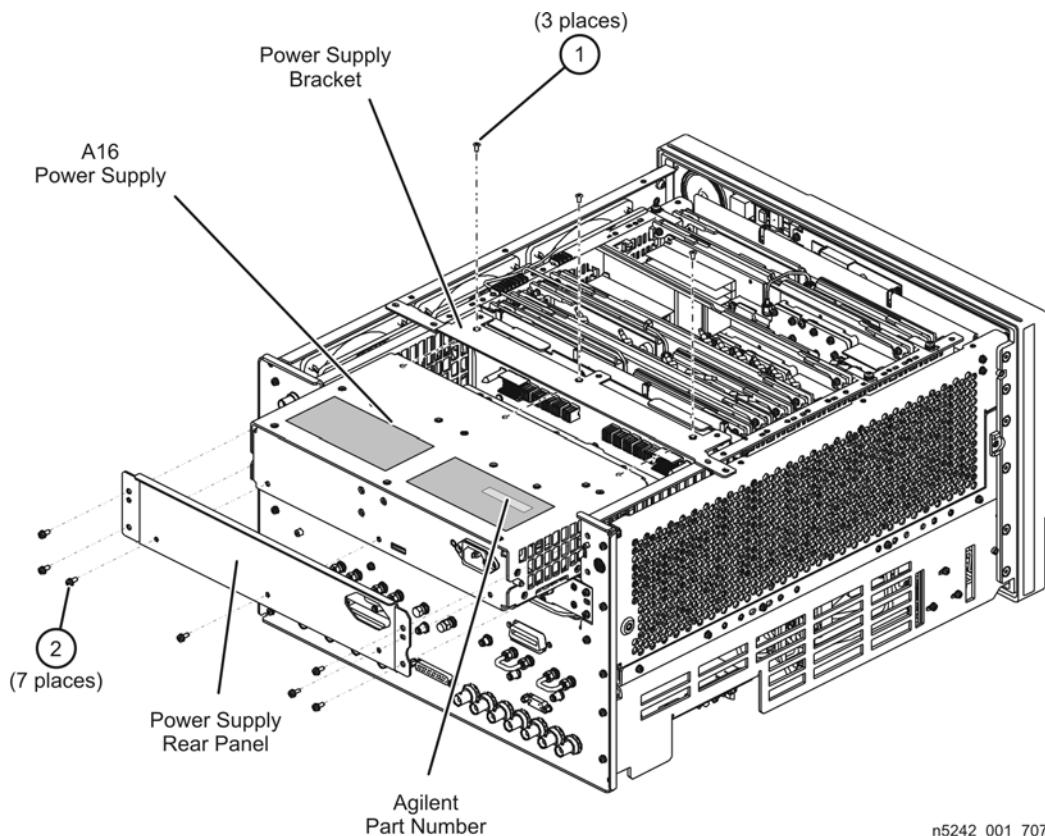
Figure 15 Power Supply Replacement
