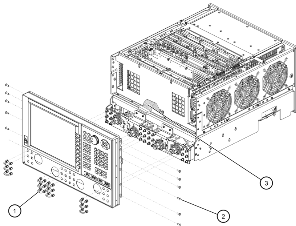
Figure 17 Front Panel Assembly Reinstallation
